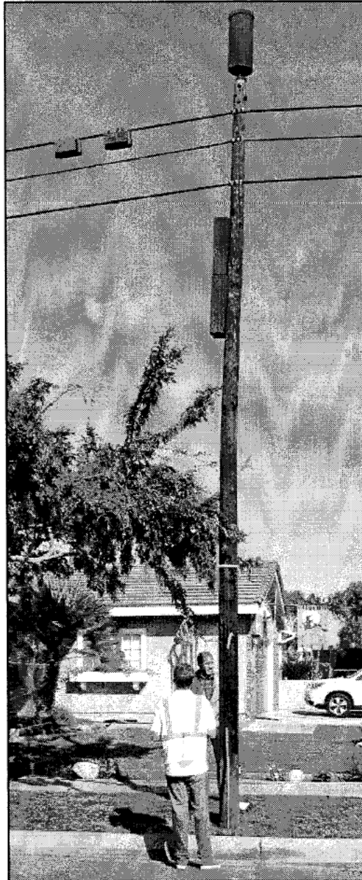
Figure 1: Omni-directional antenna, Pole-top Mount, Fiber Node, 4 DC power converters, 4 RRUs enclosed within two enclosures, RF signage (Omits materially visible elements, e.g., connecting wires, PVC conduits, etc.) (Source: Photo Simulations provided by Applicant).
