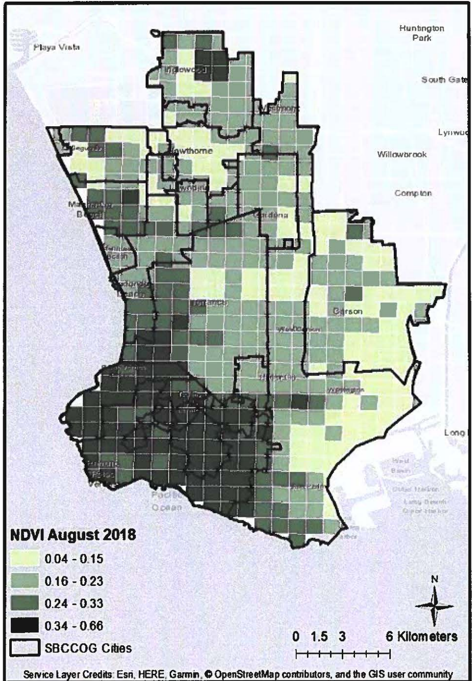
Figure 6.5 NDVI August 2018
