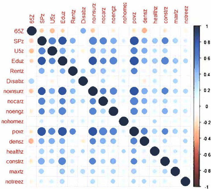
Figure 1: Correlation Matrix
